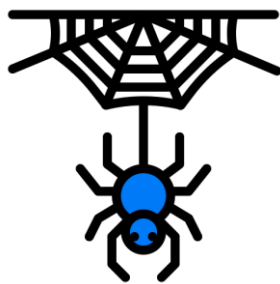
Web 거미줄
