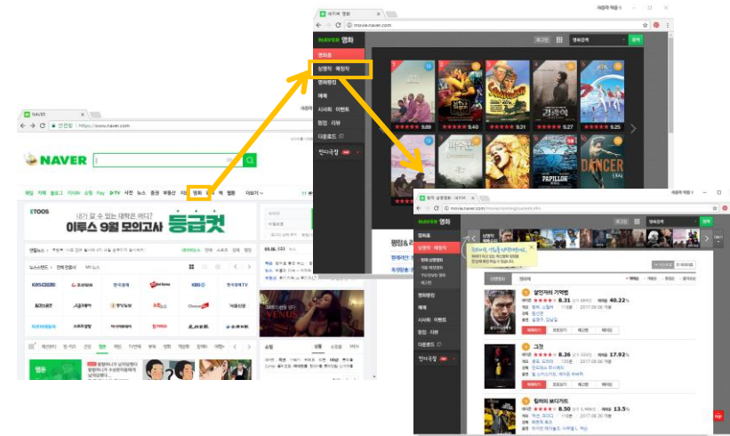
Web crawler
